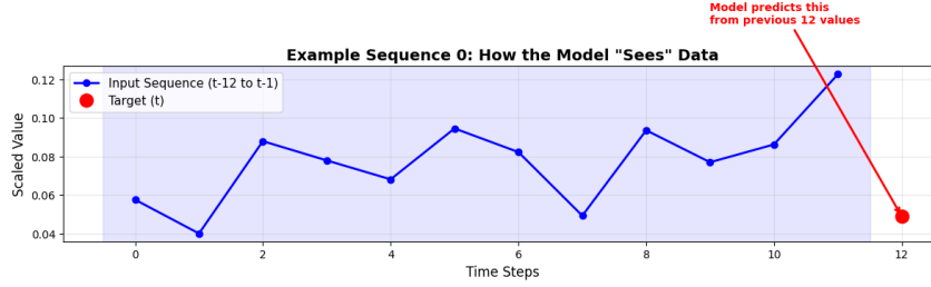
Figure 2.2: Illustration of the sliding window approach using a 12-month sequence length
