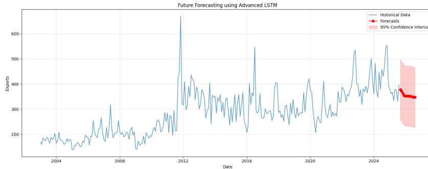
Figure 3.2: Out-of-sample export forecasts generated using the Advanced LSTM with a 12-month sliding window approach
