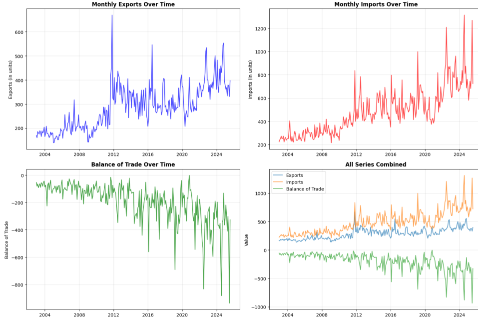
Figure 2.1: Plot of Exports, Imports and Balance of Trade
