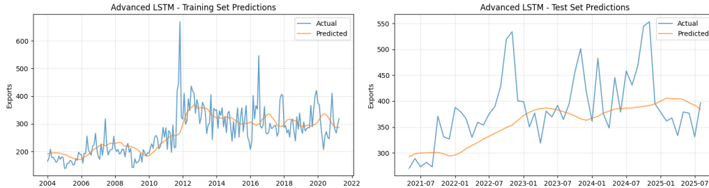
Figure 3.1: Actual and predicted monthly export values for the Advanced LSTM with a 12-month sequence length on the training and test datasets
